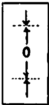
Fig. 7 Simultaneous reactions
