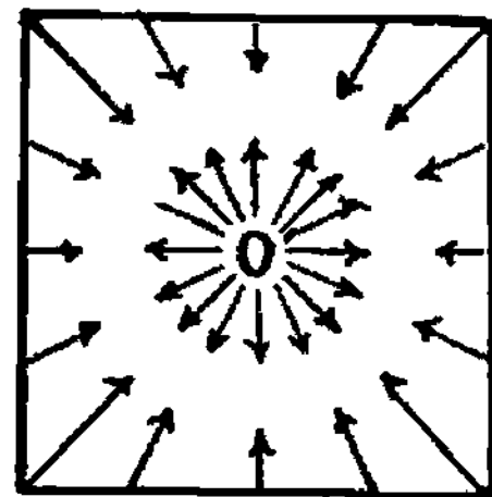
Fig. 8 Sequential reaction
