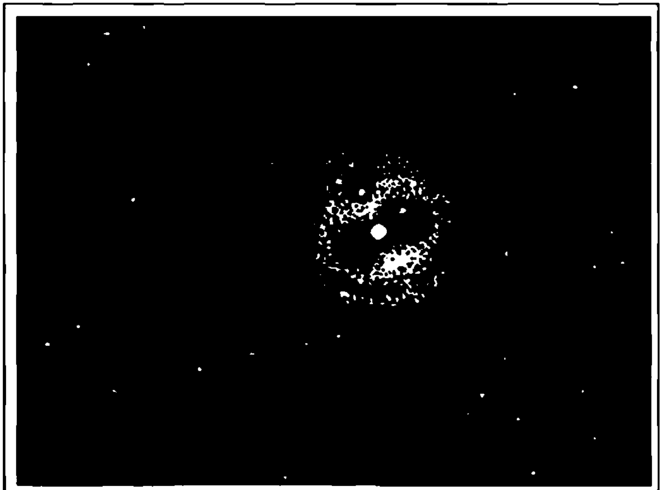
Fig. 62 Owl nebula
